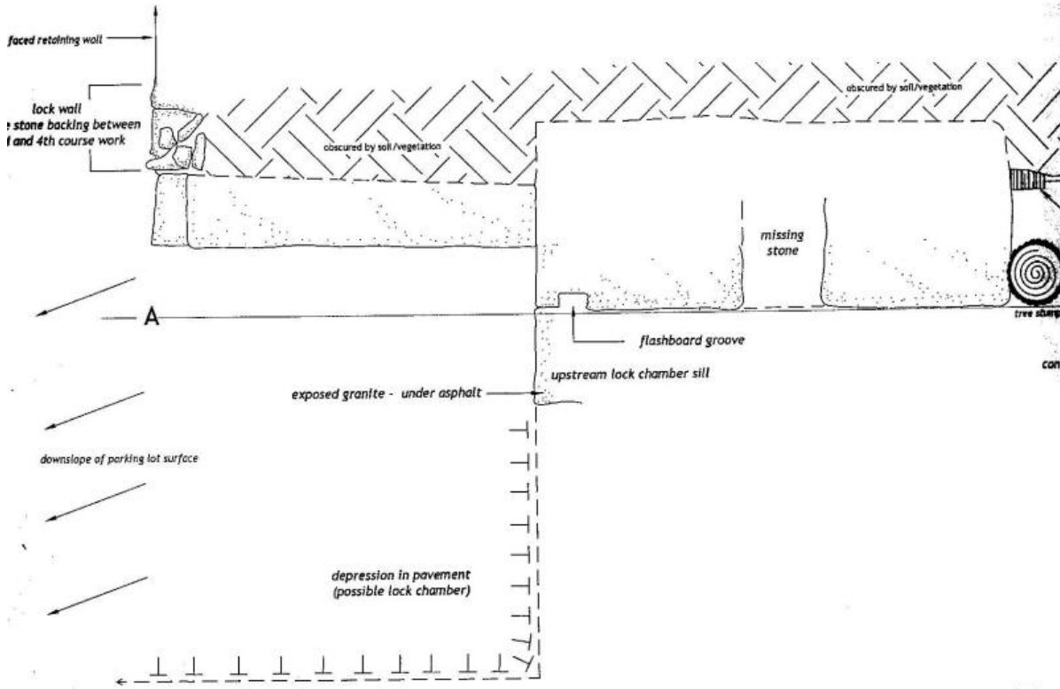
Measured plan and profile of the Blackstone Canal Lock #5, Pawtucket, RI.
