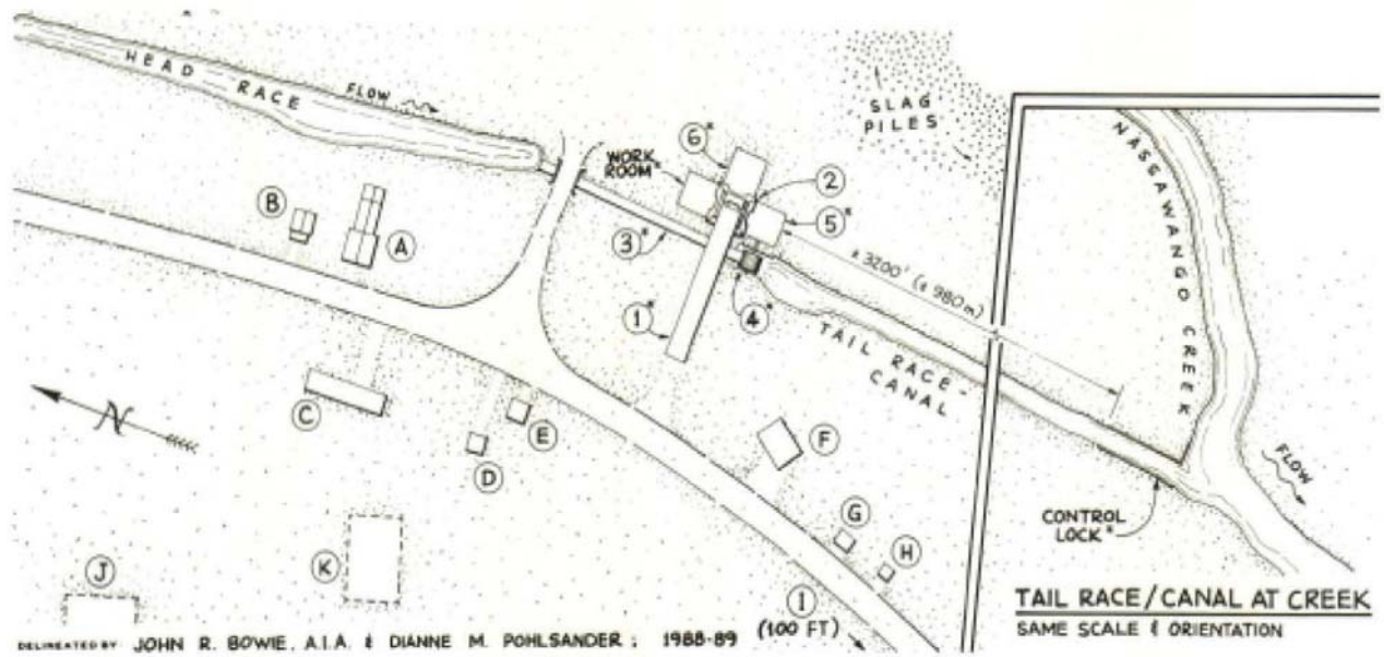
Map of the Nassawango Furnace showing the lock site from the ASME web site
